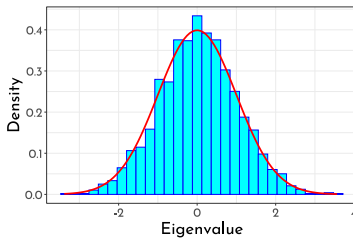
(a) \bar{G}_{p,N}(x)
