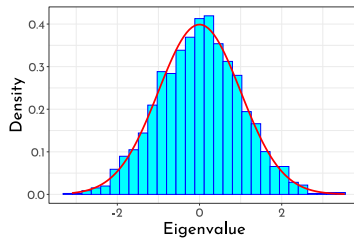
(b) \bar{G}_{p,N}(x^2)
