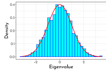
(c) \bar{G}_{p,N}(x^3)
