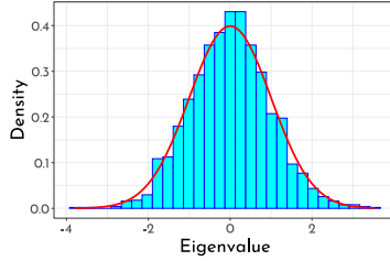
(b) \bar{G}_{p,N}(x^2)
