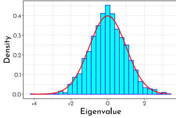
(a) \bar{G}_{p,N}(x)
