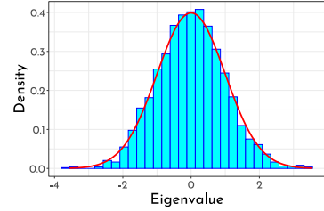
(c) \bar{G}_{p,N}(x^3)
