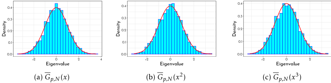
Figure 4: Histograms of normalized LSS \bar{G}_{p,N}(x^r) , r = 1, 2, 3 , with w_{ij} \sim \chi^2(1) and (p, n) = (300, 400) . The curves are density functions of the standard normal distribution.
