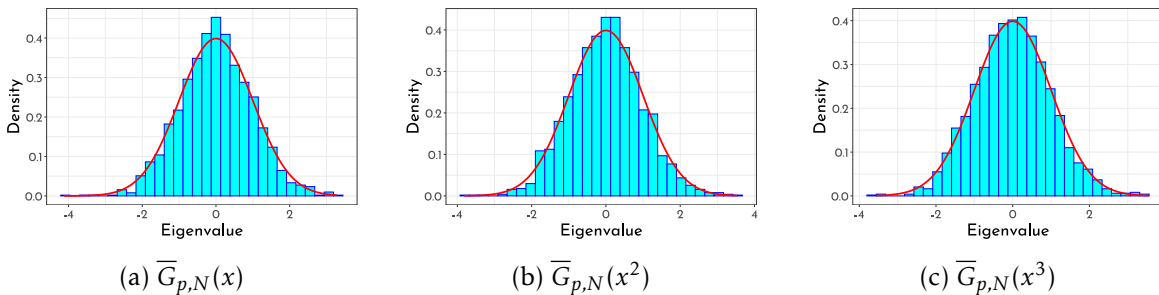
Figure 3: Histograms of normalized LSS \bar{G}_{p,N}(x^r) , r = 1, 2, 3 , with w_{ij} \sim \text{Exp}(5) and (p, n) = (400, 400) . The curves are density functions of the standard normal distribution.
