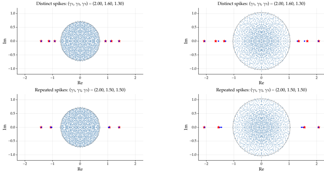
(a) Homogeneous variance profile
