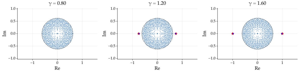
(a) Homogeneous rectangular variance profile
