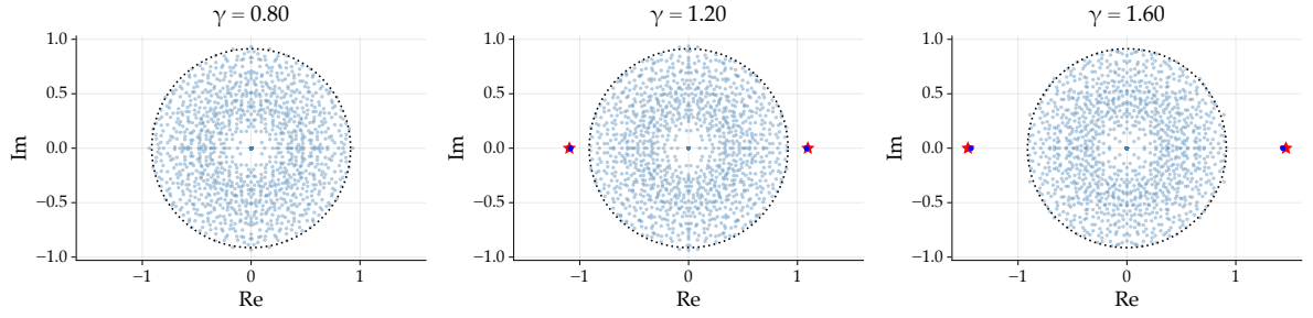
(b) Heterogeneous rectangular variance profile
