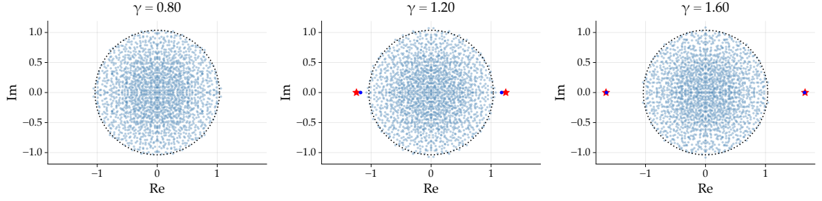
(b) Heterogeneous variance profile
