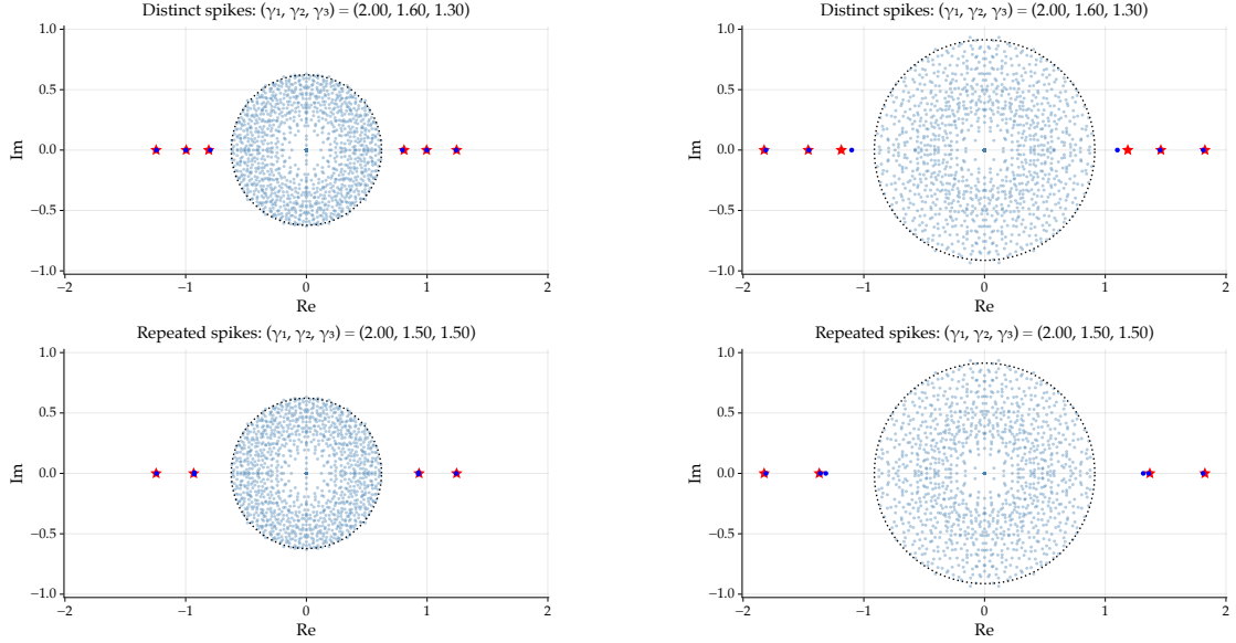
(a) Homogeneous rectangular variance profile
