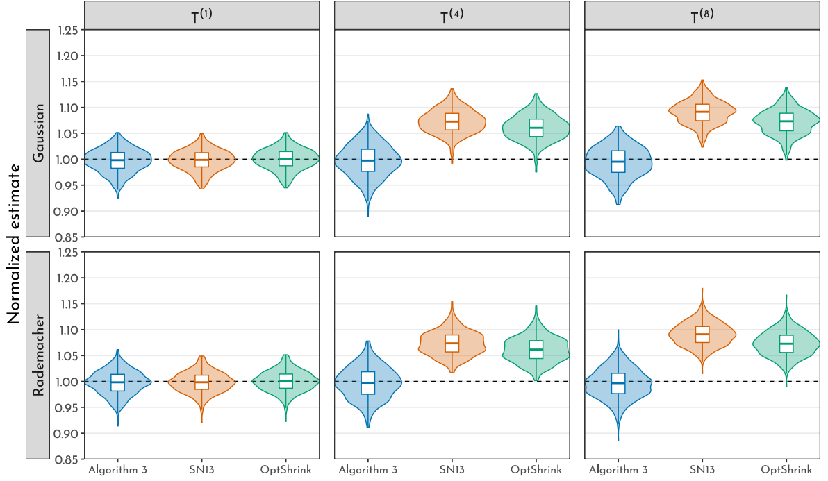
Figure 6: Violin plots of the normalized spike estimates \hat{d}_1/d_1 at (p, n) = (600, 1000) for Algorithm 3, SN13, and OptShrink under T_{\text{rec}}^{(1)} , T_{\text{rec}}^{(4)} , and T_{\text{rec}}^{(8)} , with Gaussian noise (top) and Rademacher noise (bottom). Each violin is based on B = 500 replications; the embedded boxplot shows the median and interquartile range, and the dashed horizontal line marks the target value 1. The normalized singular spike strength is \gamma = 1.50 .
