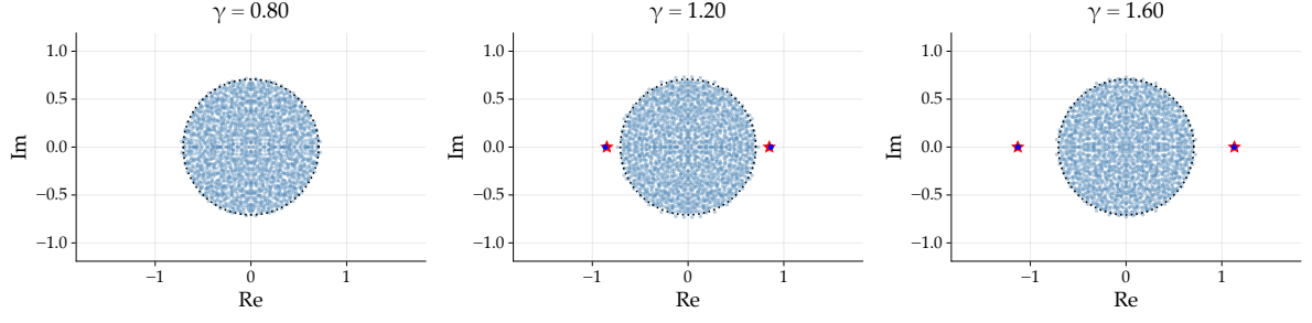
(a) Homogeneous variance profile
